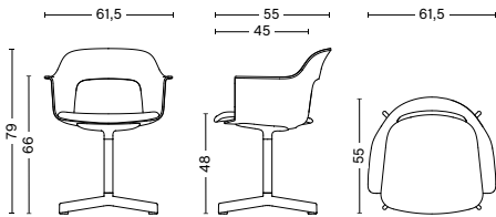
LAYOUT ARMCHAIR 234 Width 62 cm Depth 56 cm Height 80 cm Seat height 48 cm Armrest height 67 cm Weight 11,45 kg
