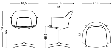
LAYOUT ARMCHAIR 232 Width 61,5 cm Depth 55 cm Height 79 cm Seat height 45,5 cm Armrest height 66 cm Weight 9,65 kg
