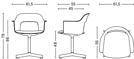
LAYOUT ARMCHAIR 233 Width 61,5 cm Depth 55 cm Height 79 cm Seat height 48 cm Armrest height 66 cm Weight 10,55 kg
